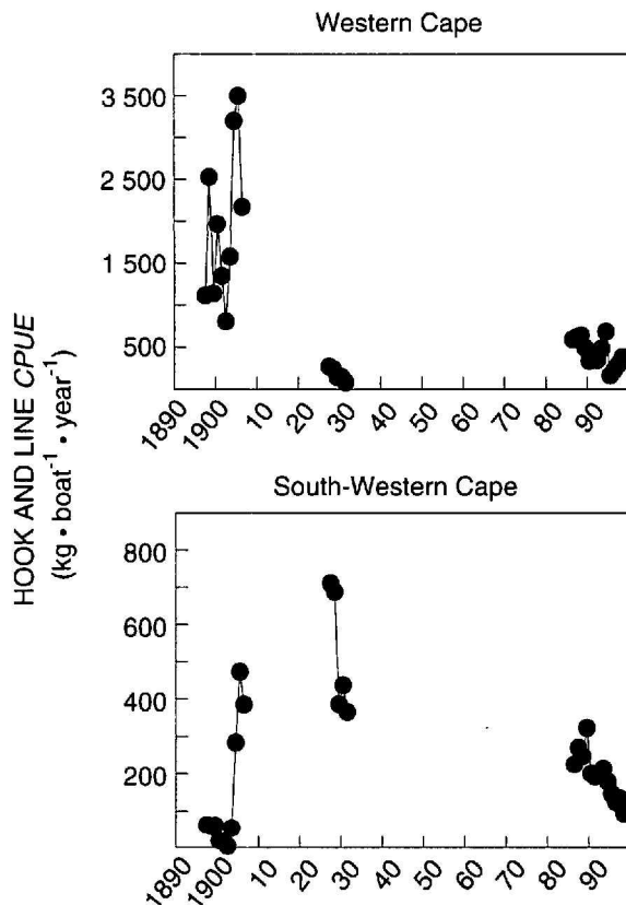
Fig. 11: Average annual cpue of hottentot caught by lineboats in Cape waters
