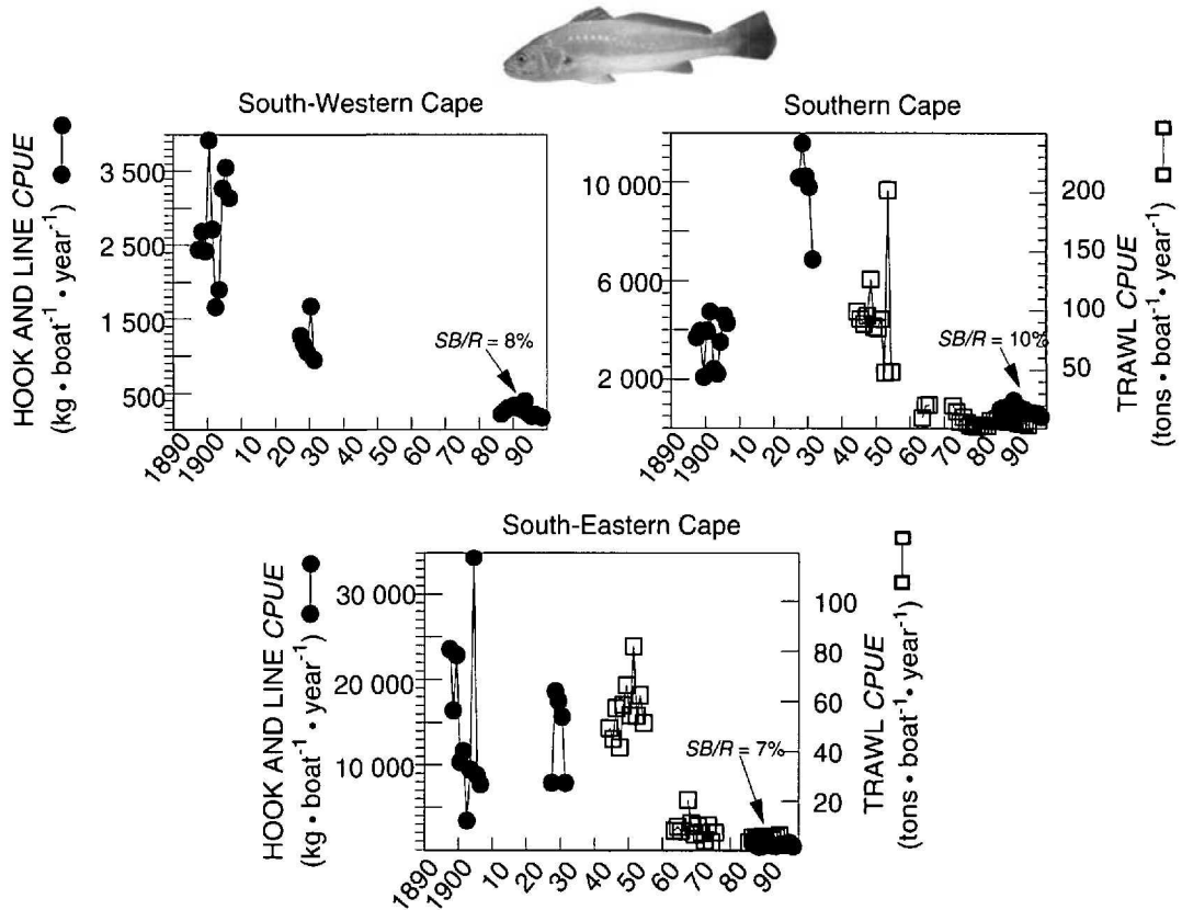
Fig. 3: Average annual cpue of three stocks of silver kob caught by lineboats and trawlers in Cape waters. SB/R values indicate current spawner biomass-per-recruit ratios calculated as a percentage of pristine (from Griffiths 1997b). Values <25% indicate stock collapse
