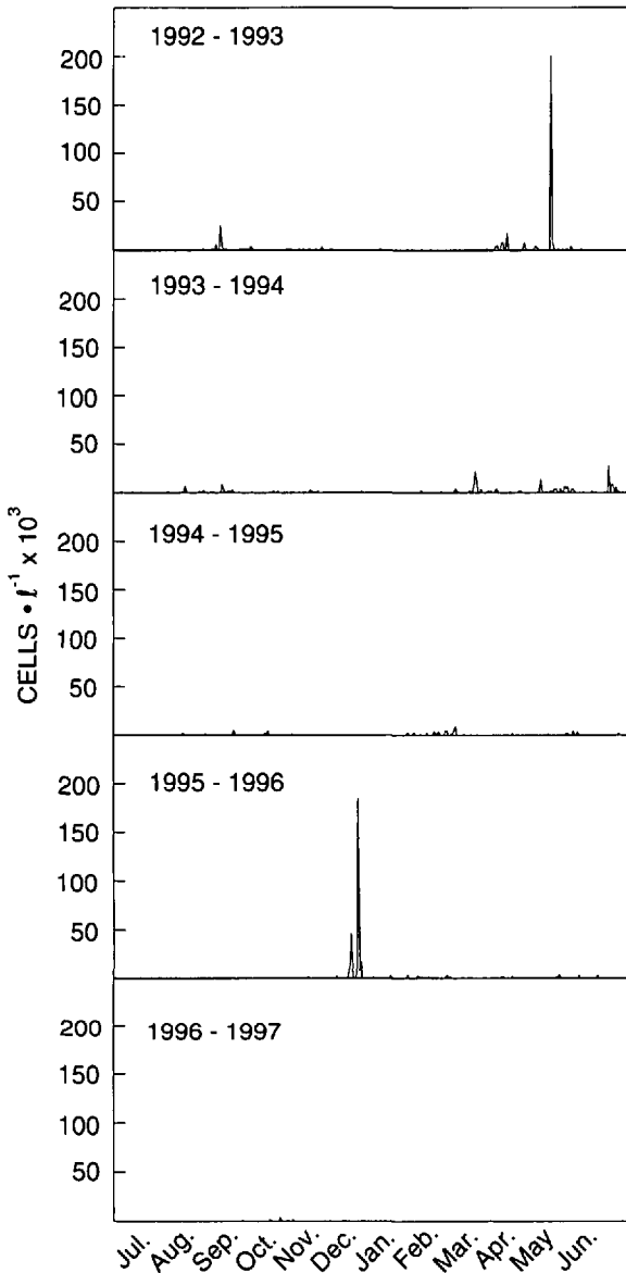
Fig. 8: Daily time-series of D. acuminata at Gordons Bay (1 July 1992–30 June 1997)
