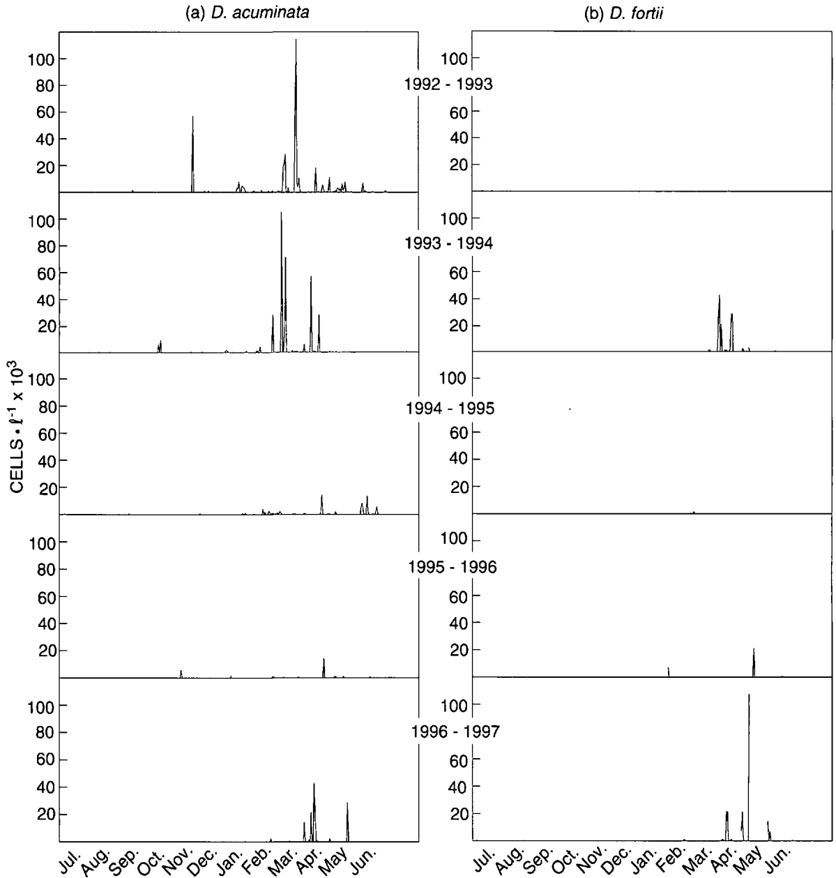
Fig. 9: Daily time-series of (a) D. acuminata and (b) D. fortii at Elands Bay (1 July 1992–30 June 1997)
