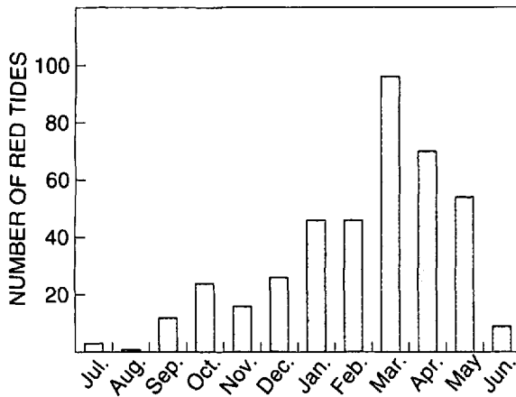
Fig. 3: Seasonal incidence of reported red tides dominated by dinoflagellates (1 July 1989–June 1997)
