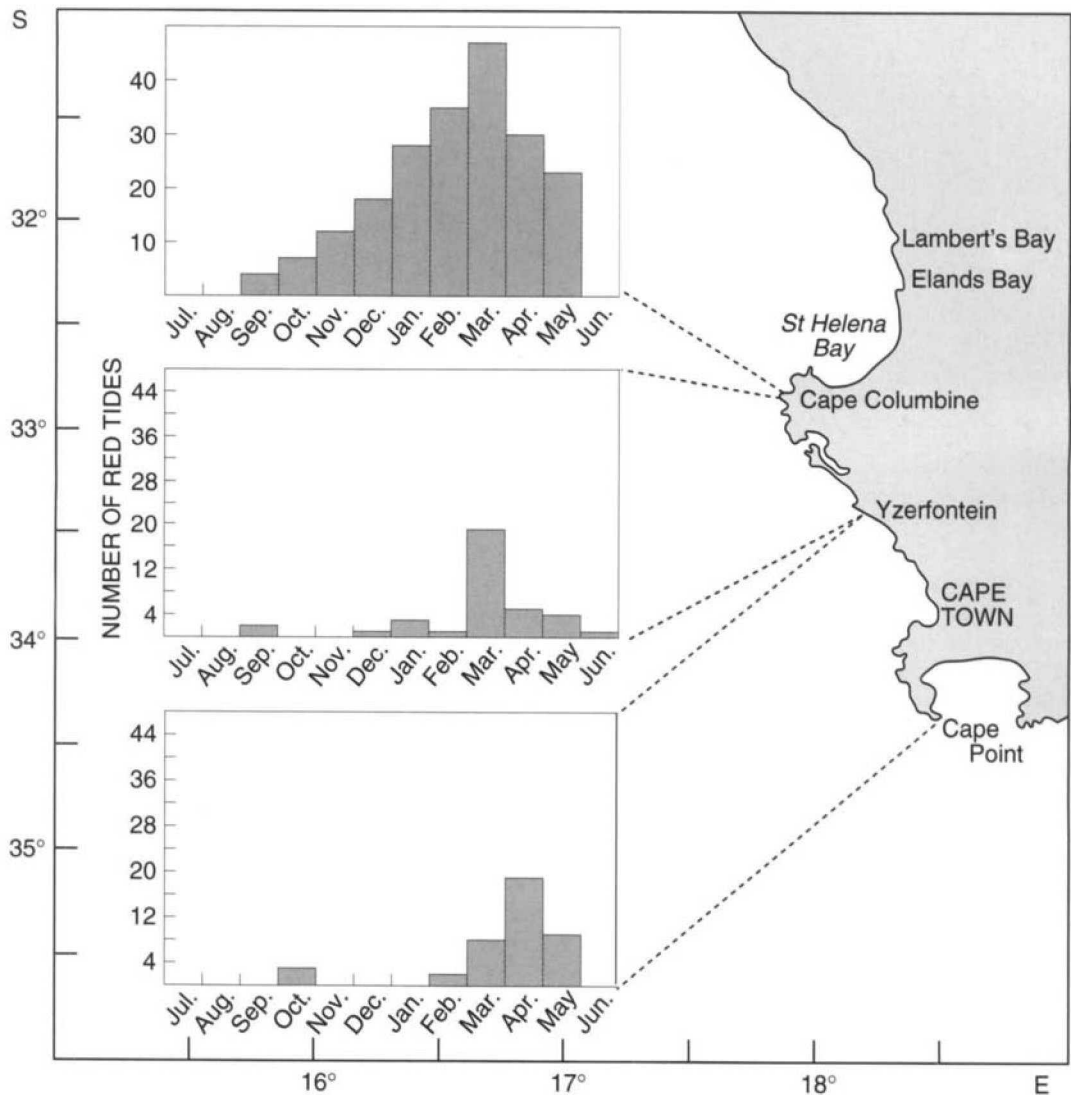
Fig. 4: Seasonal incidence of reported red tides dominated by dinoflagellates for three sectors of the West Coast (1 July 1989–30 June 1997)
