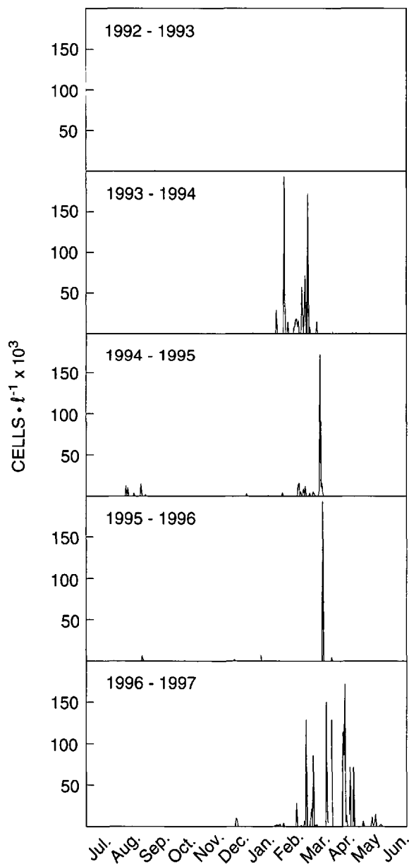
Fig. 7: Daily time-series of Alexandrium catenella at Elands Bay (1 July 1992–30 June 1997)
