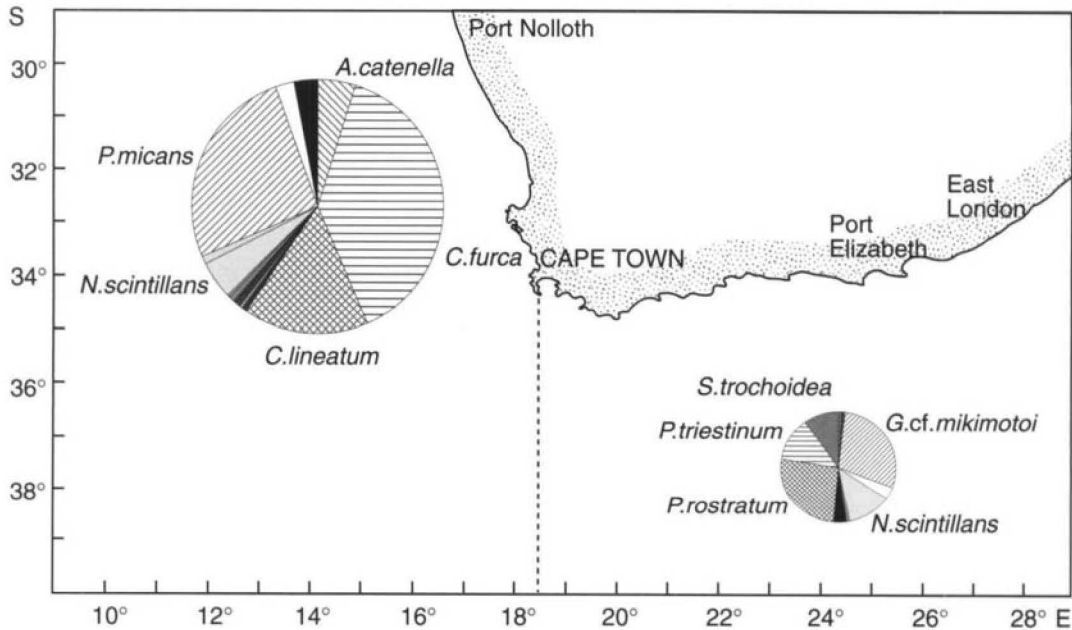
Fig. 6: Composition of reported red tides dominated by dinoflagellates on the West and South coasts (1 July 1989 to 30 June 1997)
