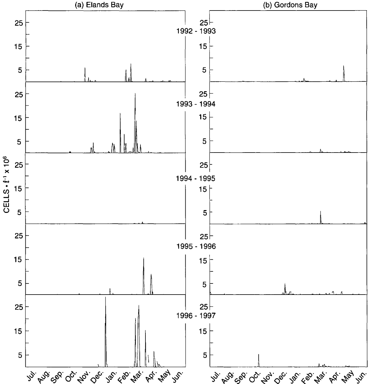
Fig. 5: Daily time-series of dinoflagellate abundance at (a) Elands Bay and (b) Gordons Bay (1 July 1992–30 June 1997)
